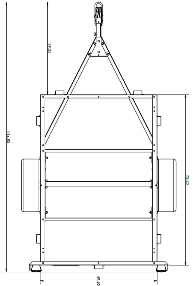
Top View
