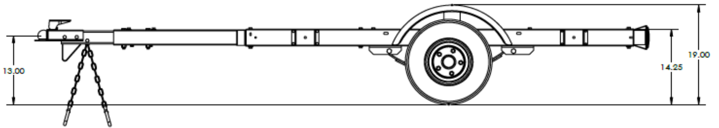
Side View
